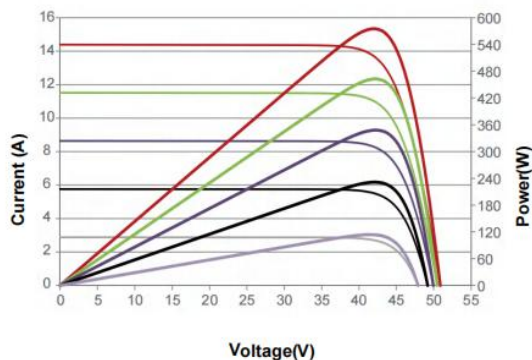
Current-Voltage & Power-Voltage Curve (GEP-DfMc580NH)
