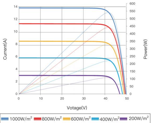
Current-Voltage & Power-Voltage Curve (GEP-DfMc550MH)
