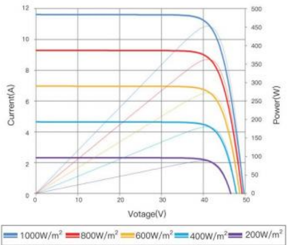
Current-Voltage & Power-Voltage Curve (GEP-CfMc450MH)
